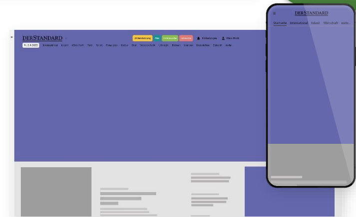
Mutation Flex
