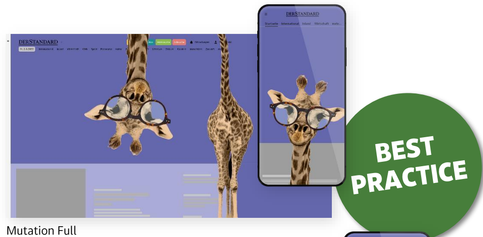
Mutation Full
